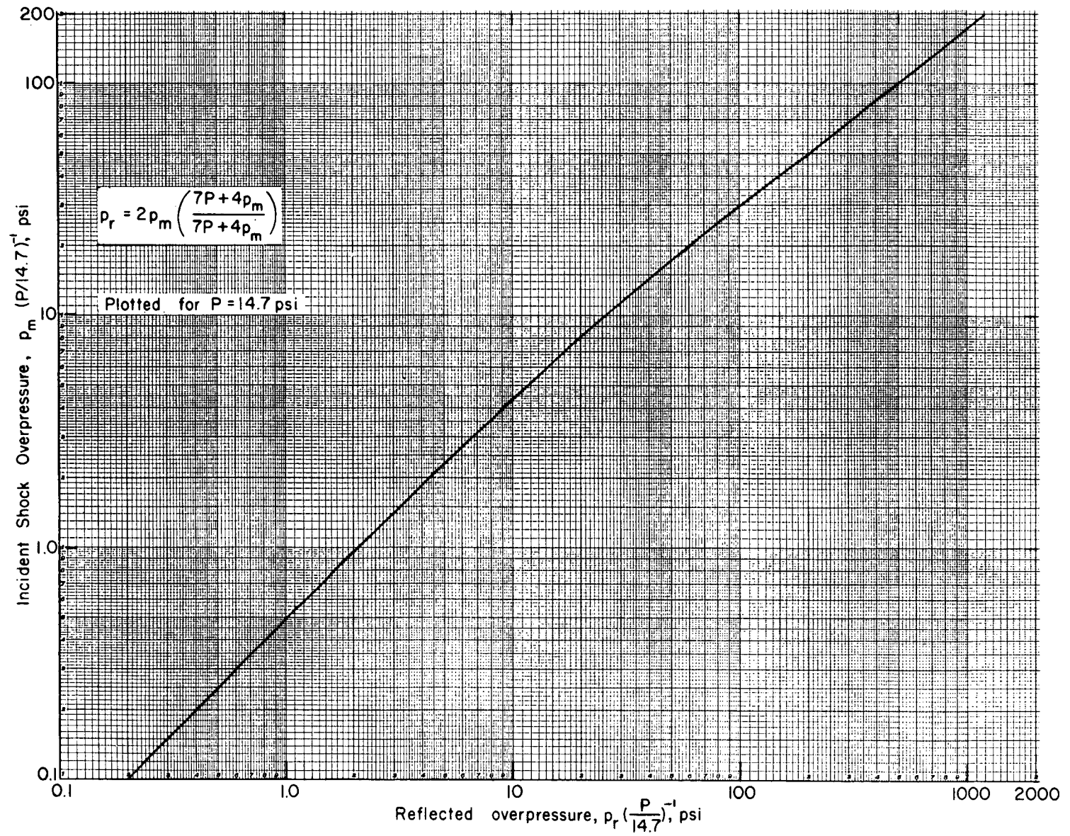
Fig. 2.10—Reflected overpressure at normal incidence as a function of incident overpressure.
